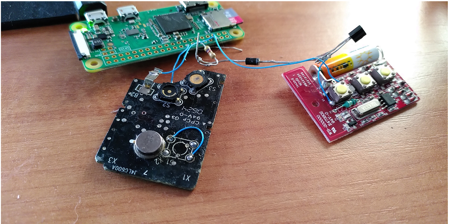
▲ Gate and garage remotes controlled by Raspberry Pi Zero
